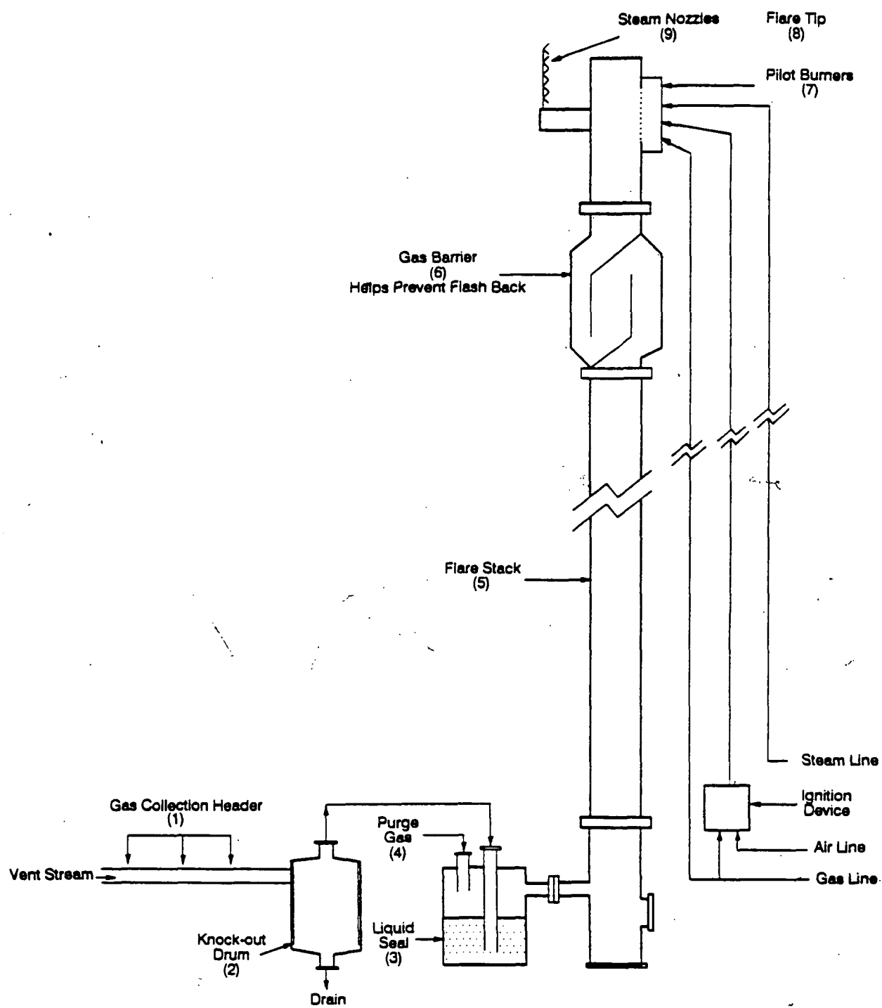
Figure 7.1: Steam-Assisted Elevated Flare System
